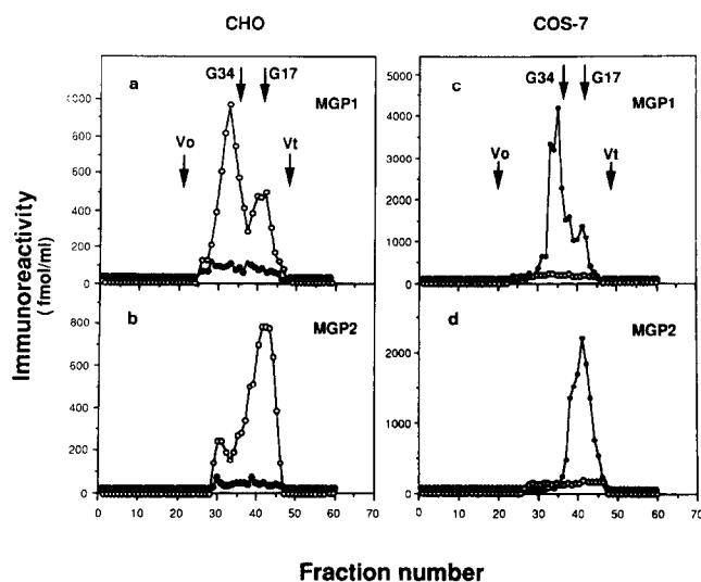
Fig. 3. Gel filtration of IRG in media from CHO and COS-7 cells transformed to express MGP1 and MGP2 DNA. (a) MGP1-expressing CHO cells; (b) MGP2-expressing CHO cells; (c) MGP1-expressing COS-7 cells; (d) MGP2-expressing COS-7 cells. IRG in eluted fractions was analyzed with the Ab5135 antibody ( \circ ) and Ab8237 antibody ( \bullet ), as described in Section 2. Columns were calibrated with blue dextran (Vo), potassium ferricyanide (Vt), and standard G17-NH 2 and G34-NH 2 . Similar chromatograms were obtained in at least three other experiments for each cell line.
